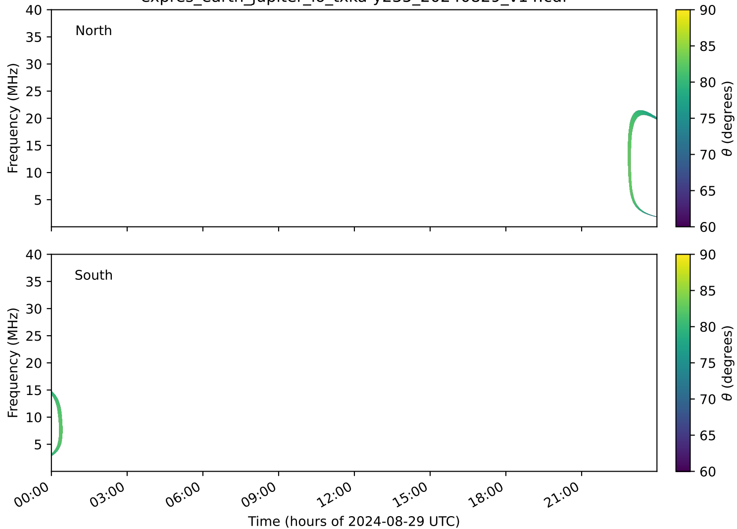
expres_earth_jupiter_io_txka-y235_20240829_v14.cdf
