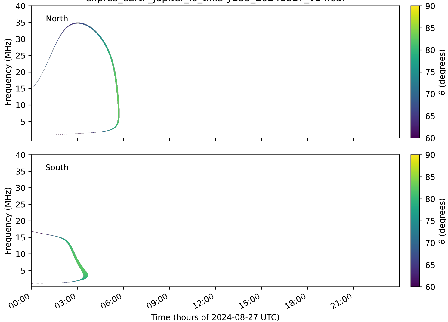
expres_earth_jupiter_io_txka-y235_20240827_v14.cdf
