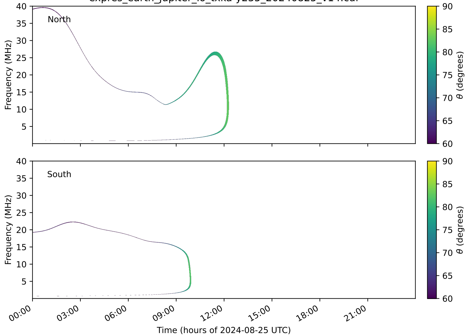
expres_earth_jupiter_io_txka-y235_20240825_v14.cdf
