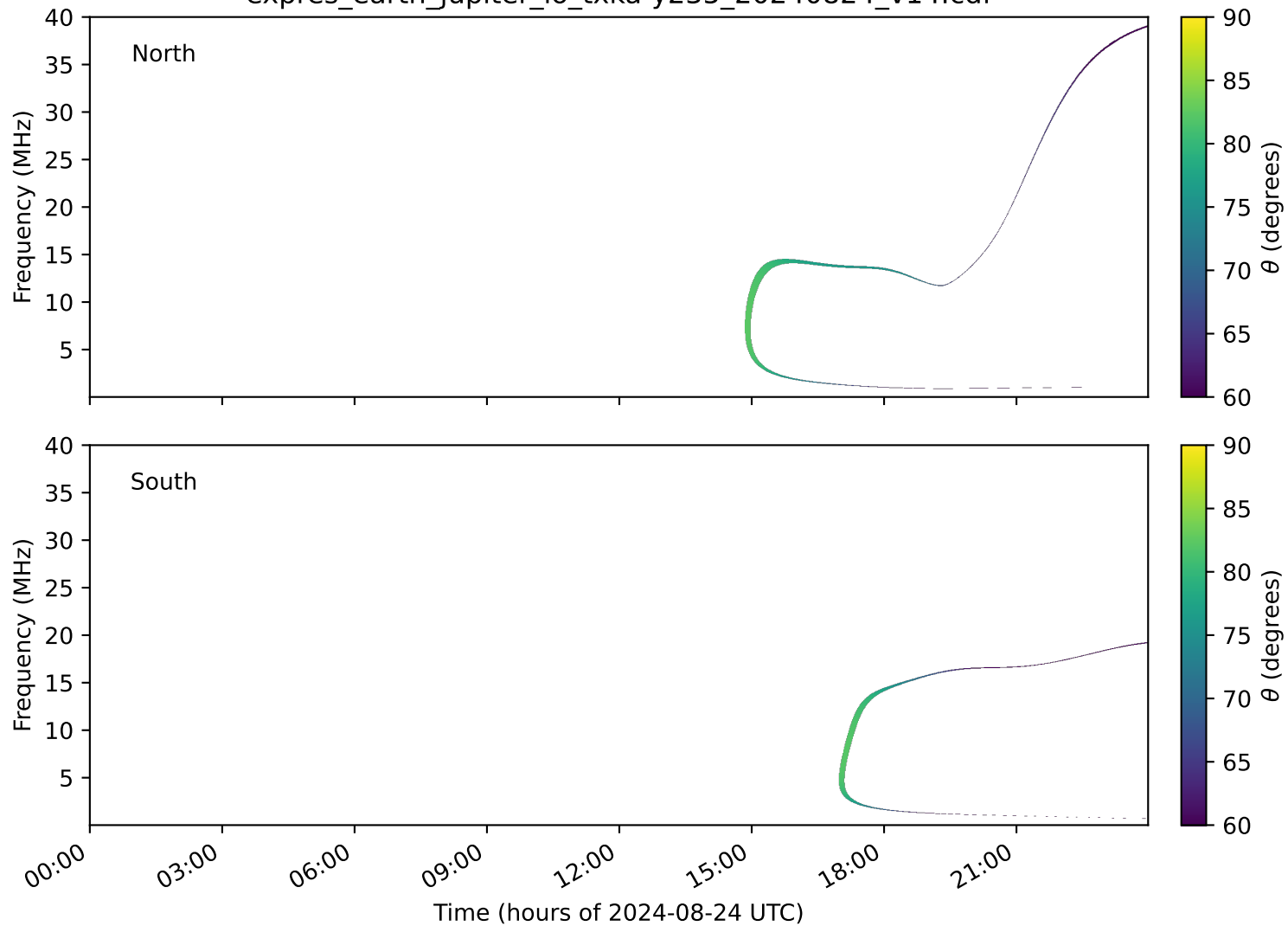
expres_earth_jupiter_io_txka-y235_20240824_v14.cdf
