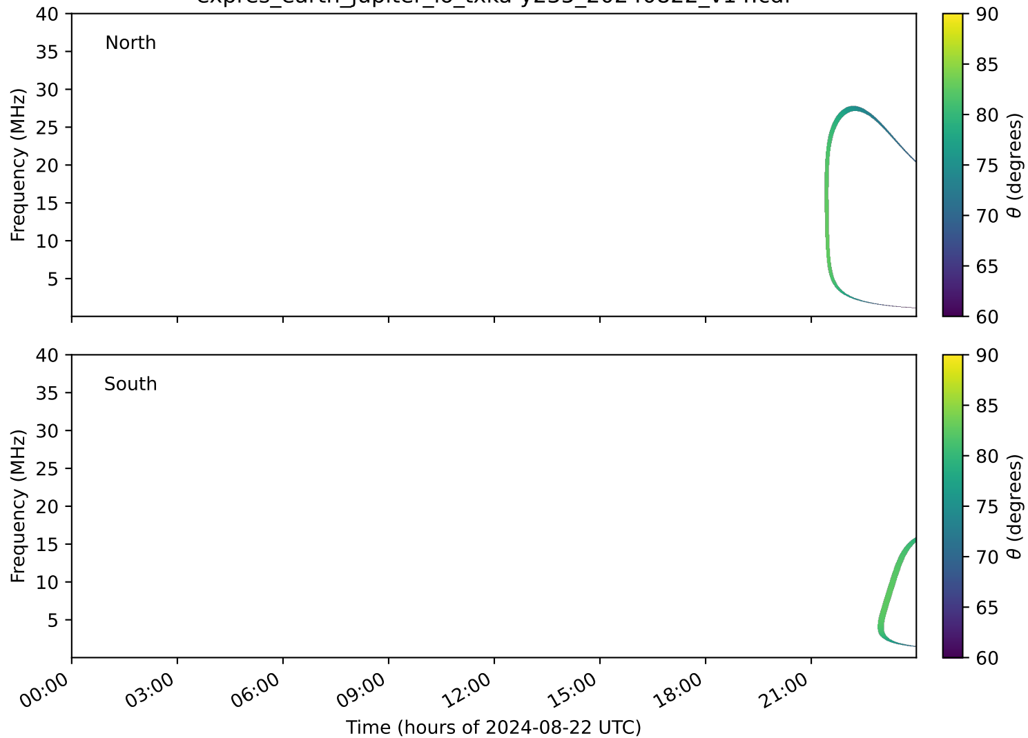
expres_earth_jupiter_io_txka-y235_20240822_v14.cdf
