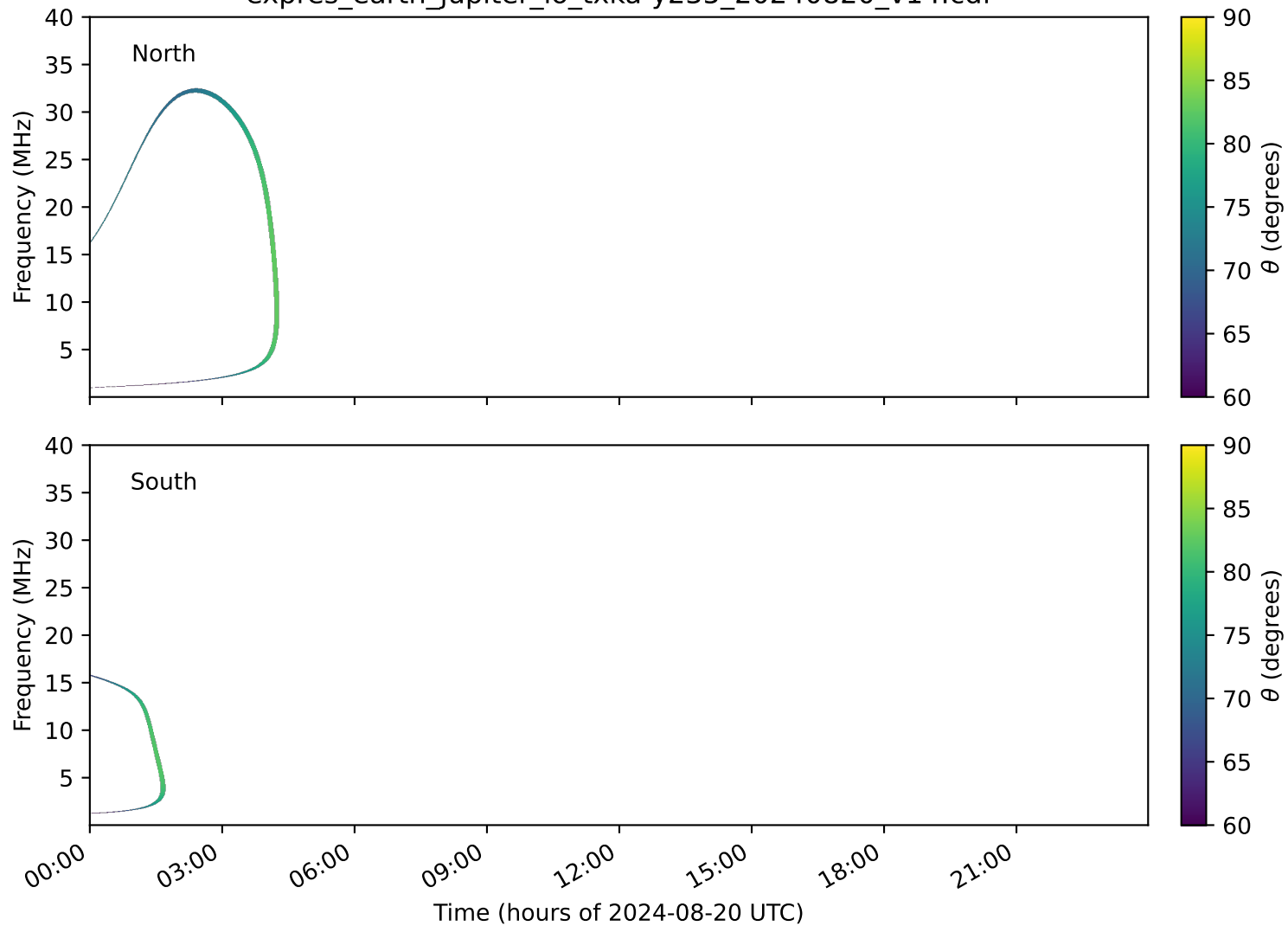
expres_earth_jupiter_io_txka-y235_20240820_v14.cdf
