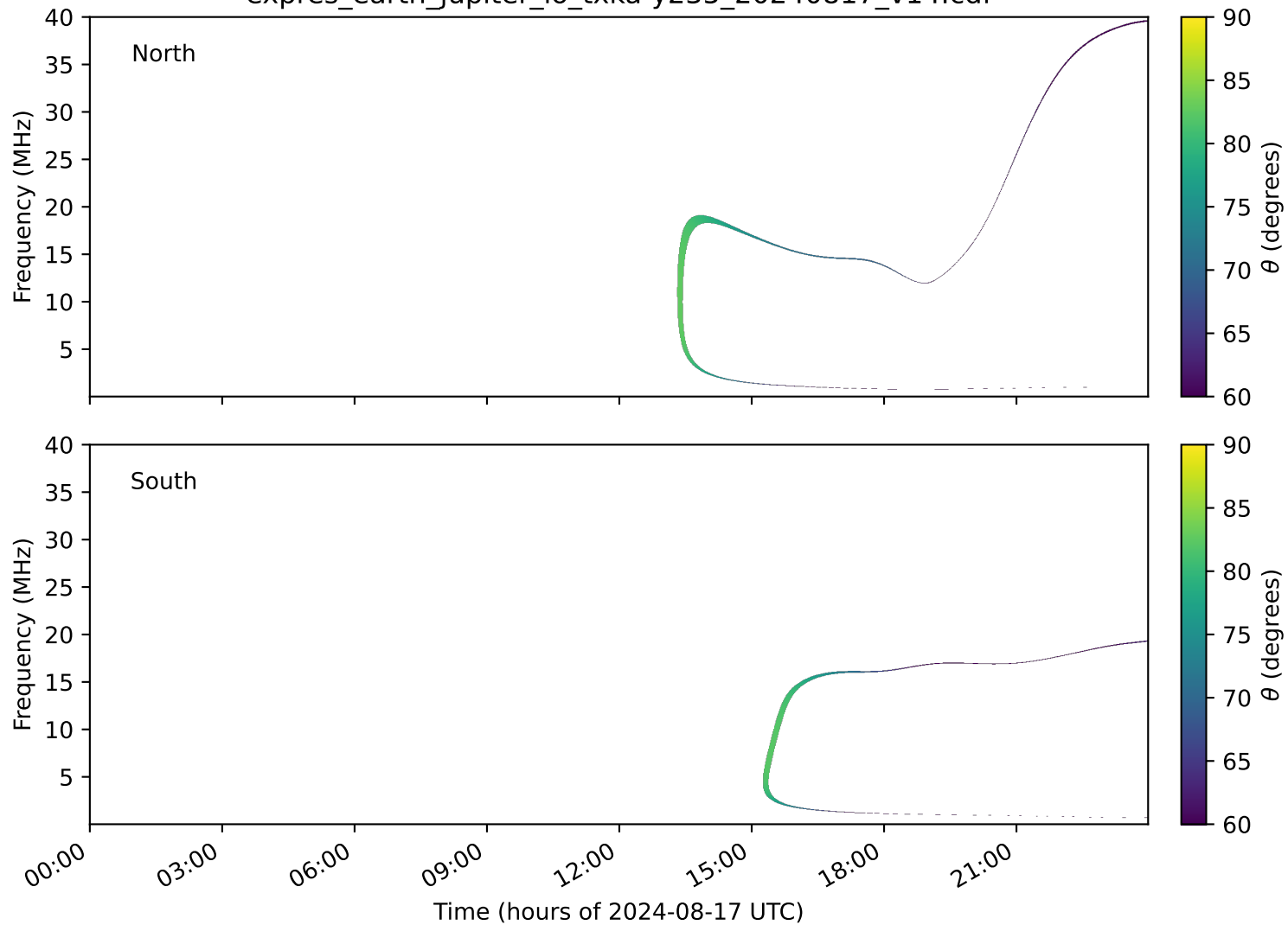
expres_earth_jupiter_io_txka-y235_20240817_v14.cdf
