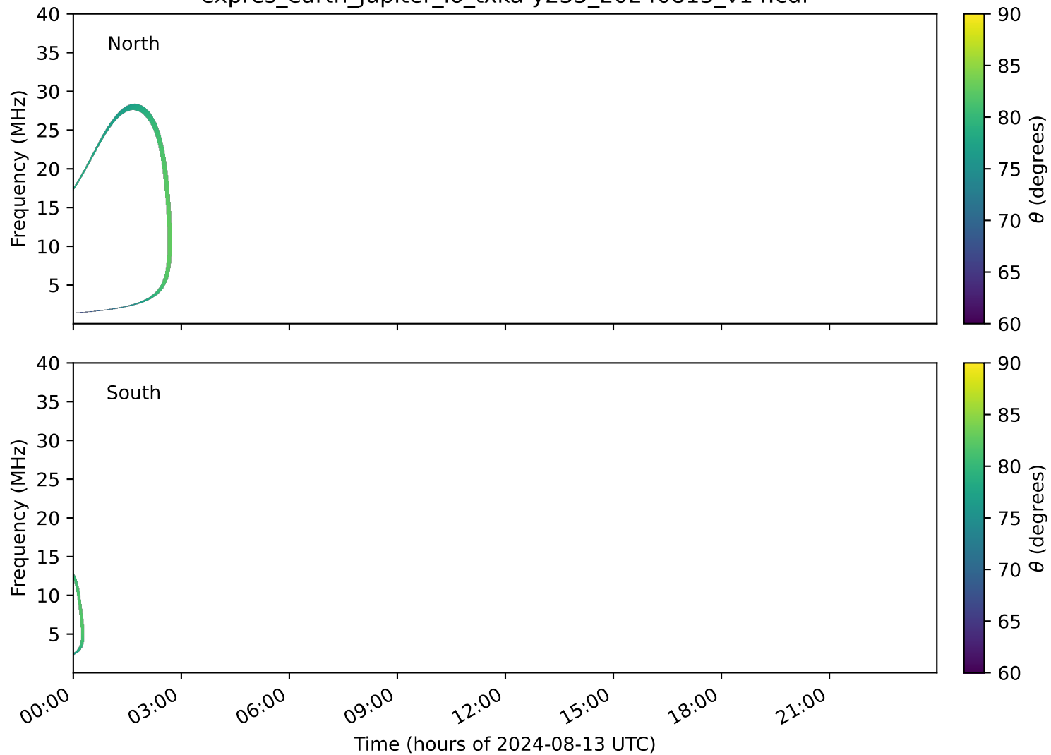
expres_earth_jupiter_io_txka-y235_20240813_v14.cdf
