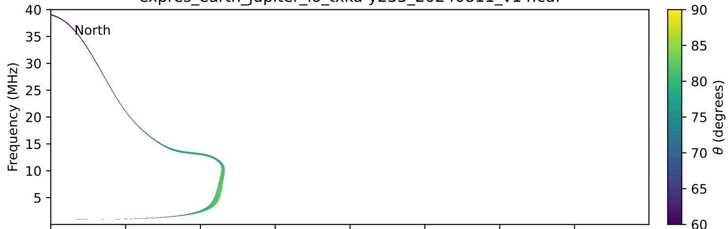
expres_earth_jupiter_io_txka-y235_20240811_v14.cdf
