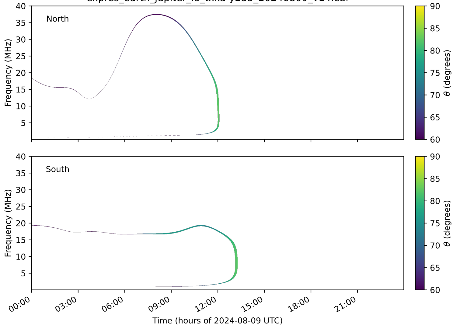
expres_earth_jupiter_io_txka-y235_20240809_v14.cdf
