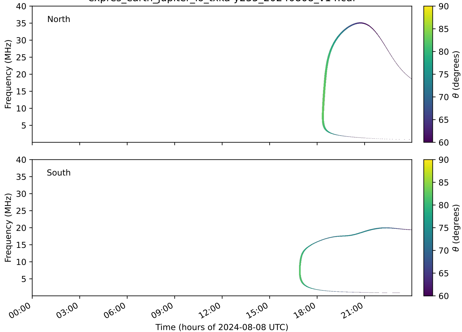
expres_earth_jupiter_io_txka-y235_20240808_v14.cdf
