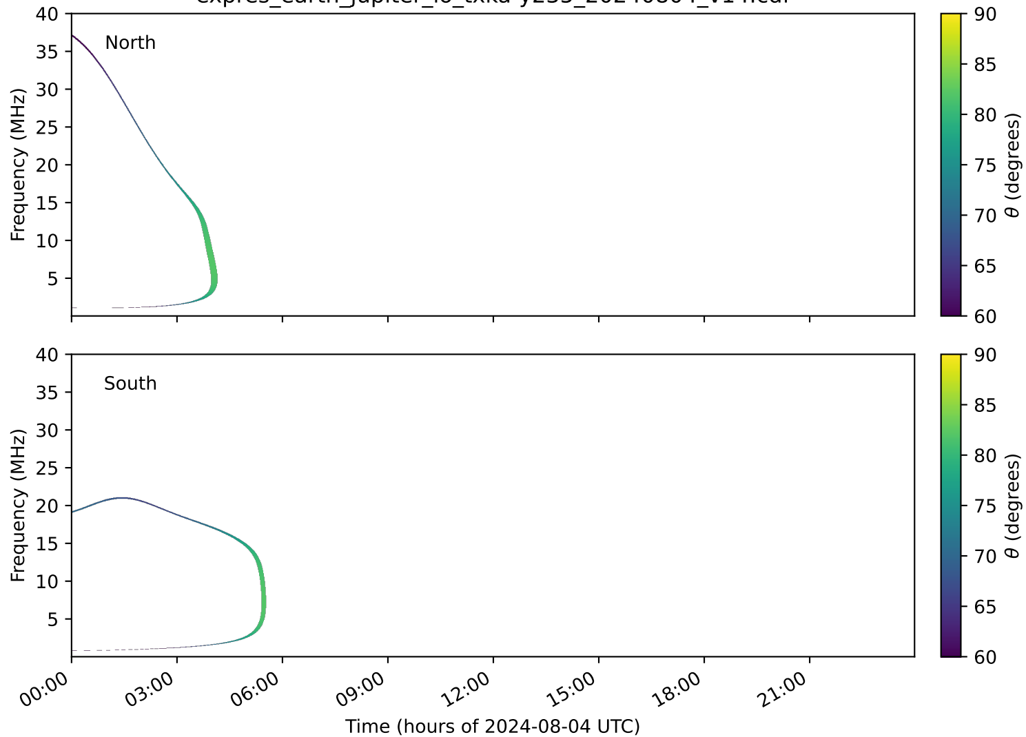
expres_earth_jupiter_io_txka-y235_20240804_v14.cdf
