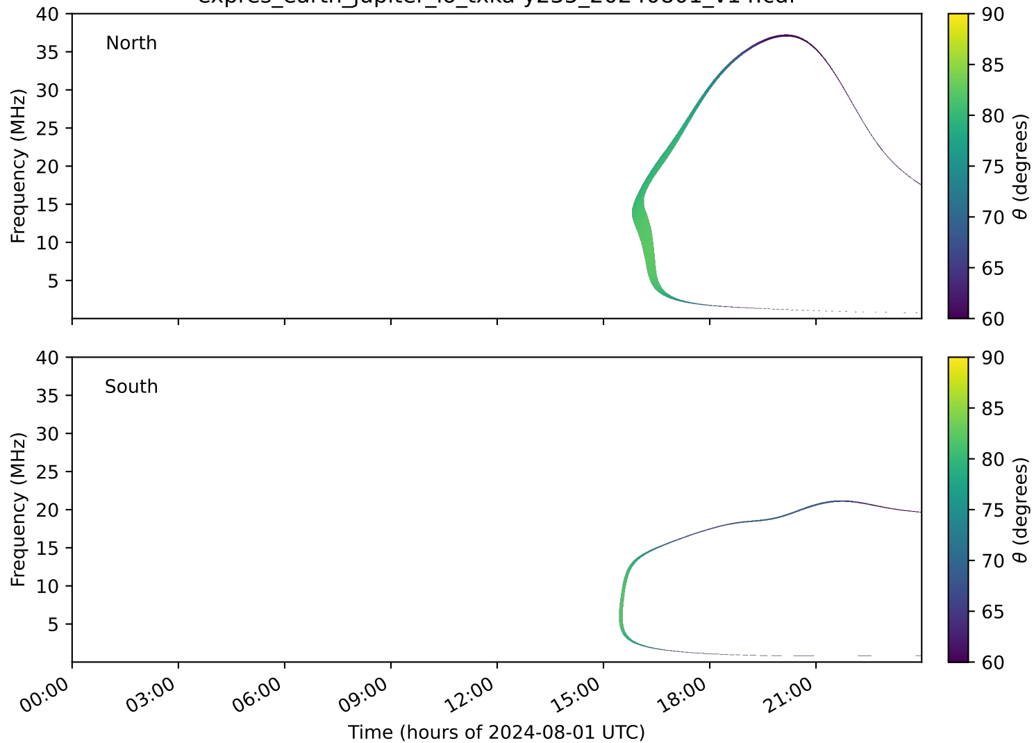
expres_earth_jupiter_io_txka-y235_20240801_v14.cdf
