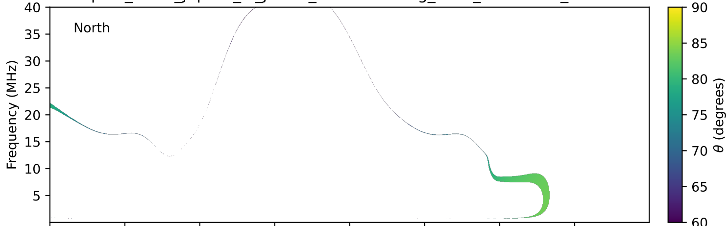
expres_earth_jupiter_io_jrm33_lossc-wid1deg_3kev_20240830_v11.cdf
