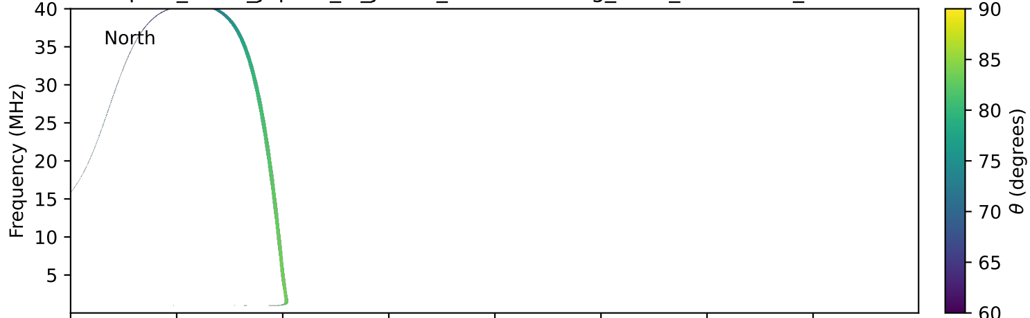
expres_earth_jupiter_io_jrm33_lossc-wid1deg_3kev_20240827_v11.cdf
