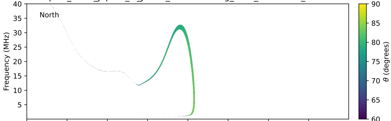
expres_earth_jupiter_io_jrm33_lossc-wid1deg_3kev_20240825_v11.cdf
