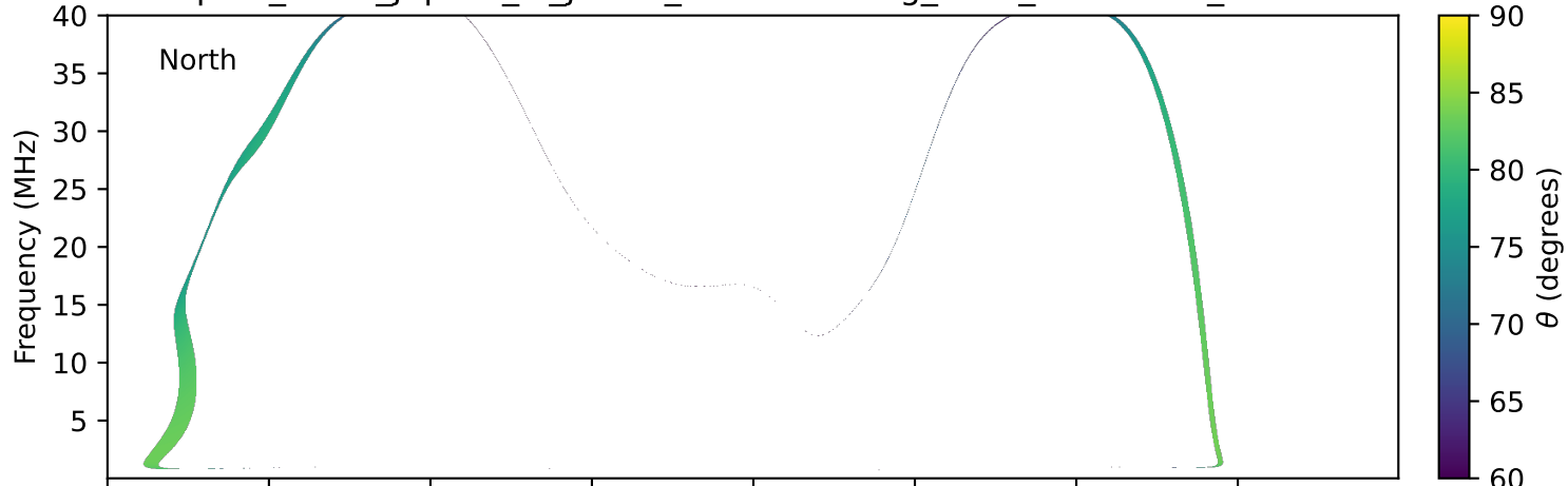
expres_earth_jupiter_io_jrm33_lossc-wid1deg_3kev_20240814_v11.cdf
