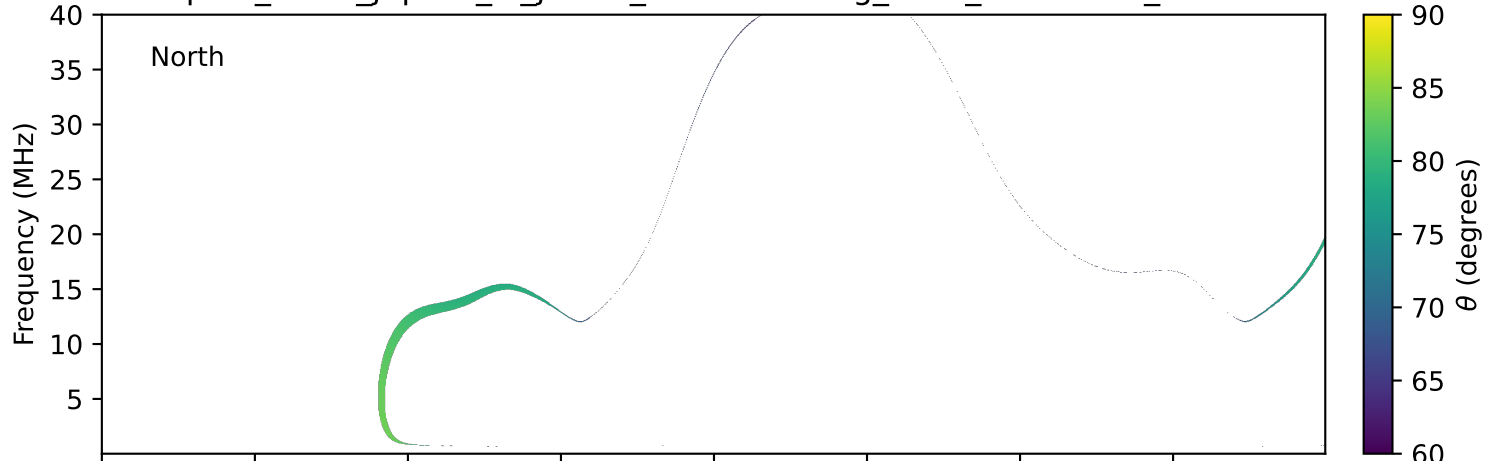
expres_earth_jupiter_io_jrm33_lossc-wid1deg_3kev_20240812_v11.cdf
