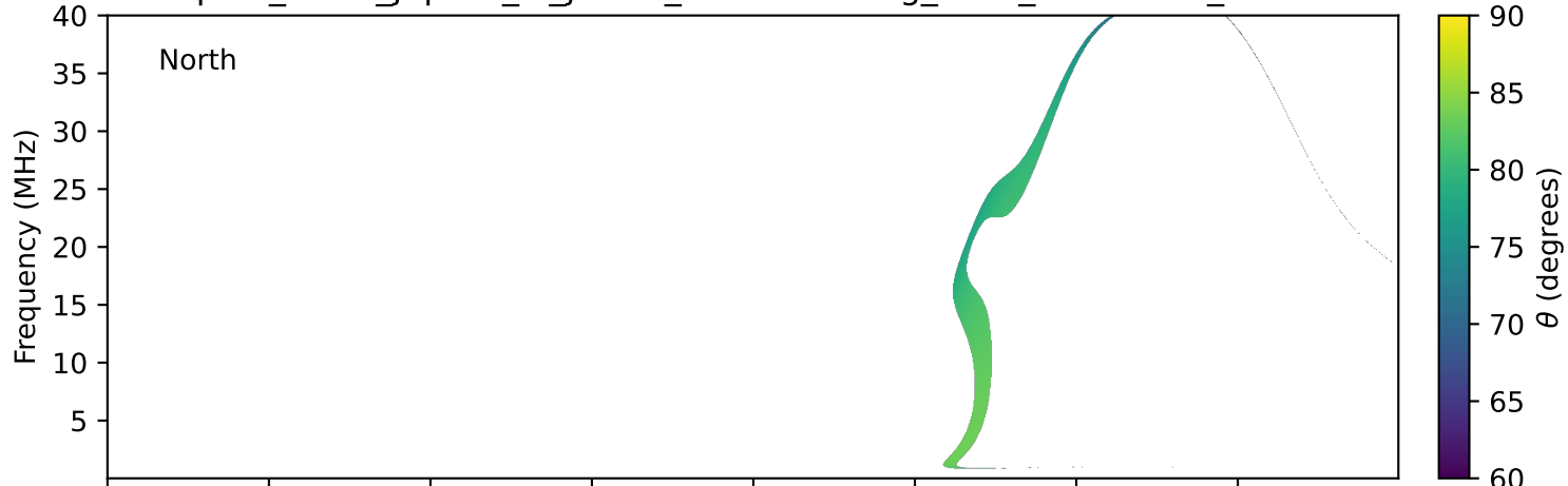
expres_earth_jupiter_io_jrm33_lossc-wid1deg_3kev_20240801_v11.cdf
