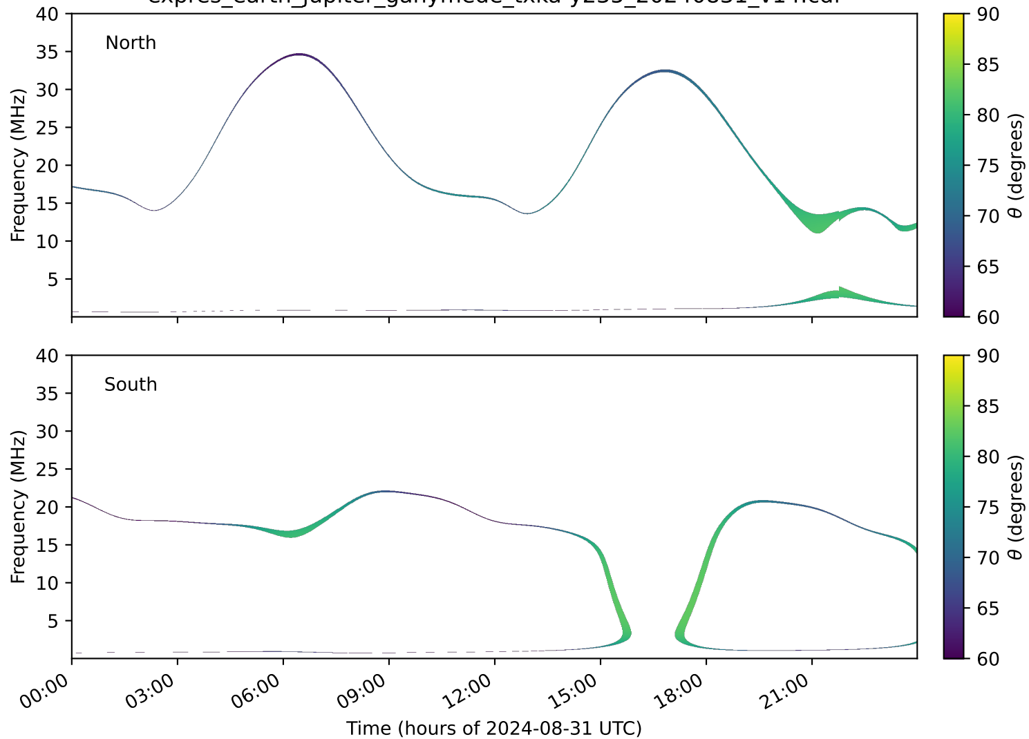
expres_earth_jupiter_ganymede_txka-y235_20240831_v14.cdf
