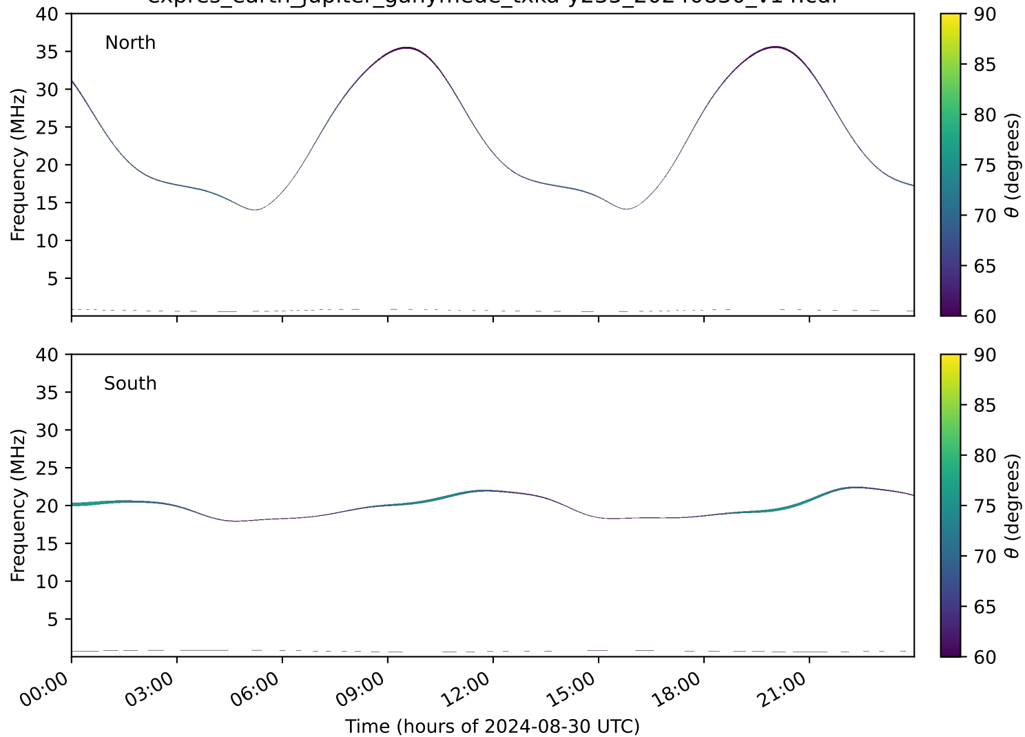
expres_earth_jupiter_ganymede_txka-y235_20240830_v14.cdf
