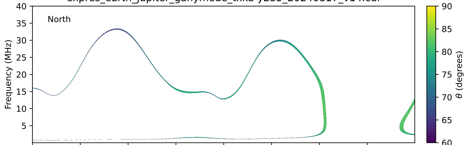
expres_earth_jupiter_ganymede_txka-y235_20240817_v14.cdf
