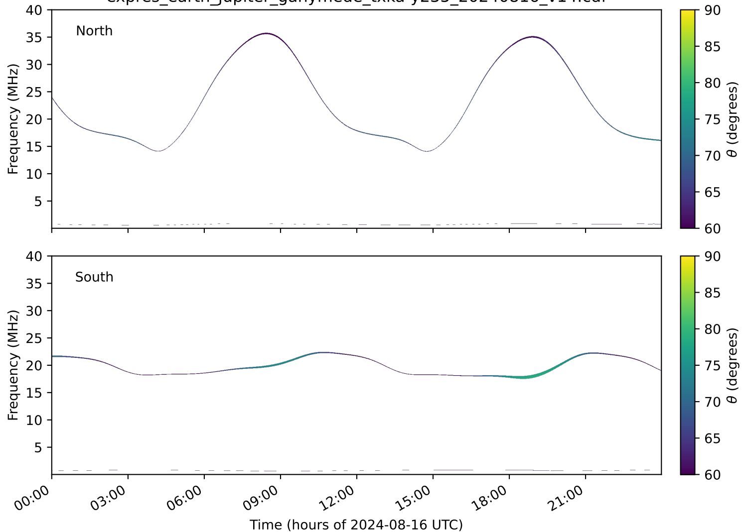
expres_earth_jupiter_ganymede_txka-y235_20240816_v14.cdf
