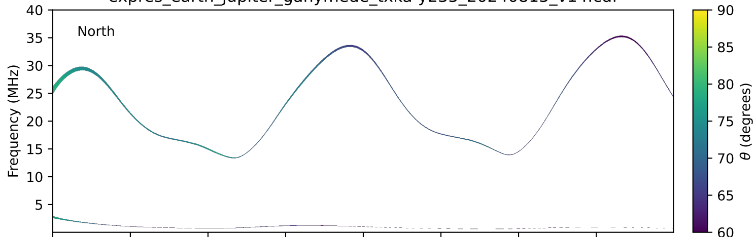
expres_earth_jupiter_ganymede_txka-y235_20240815_v14.cdf
