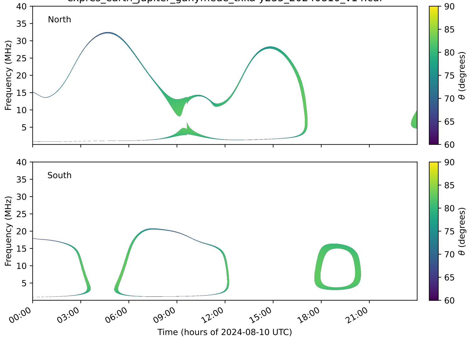
expres_earth_jupiter_ganymede_txka-y235_20240810_v14.cdf
