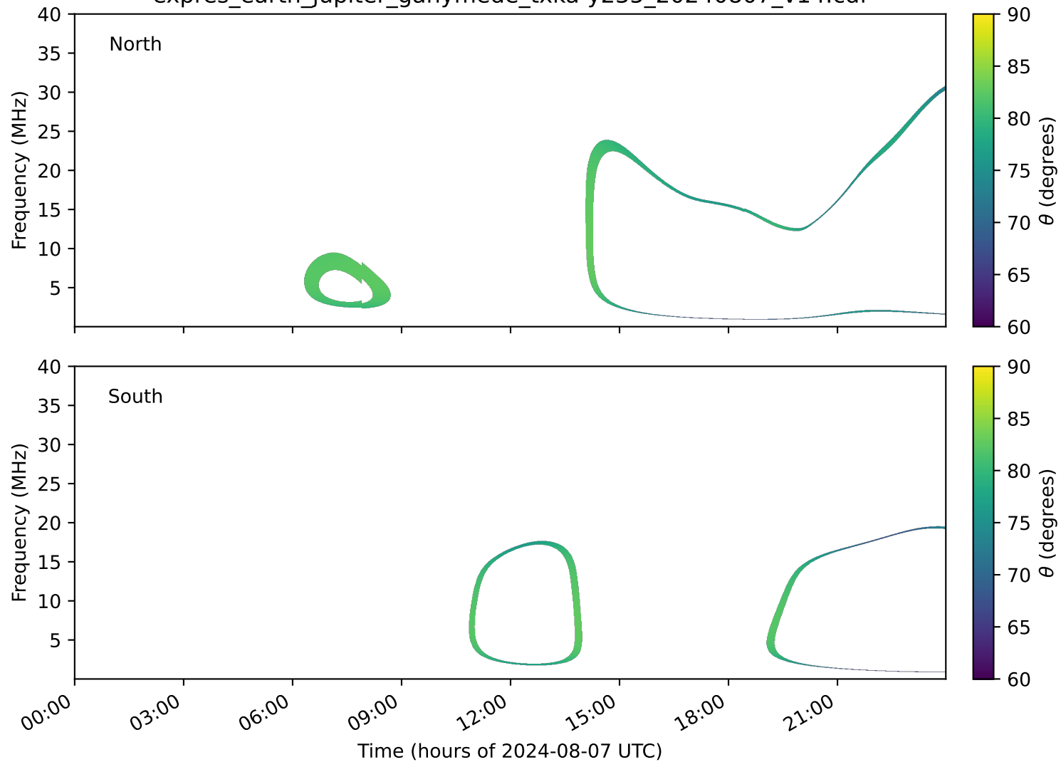
expres_earth_jupiter_ganymede_txka-y235_20240807_v14.cdf
