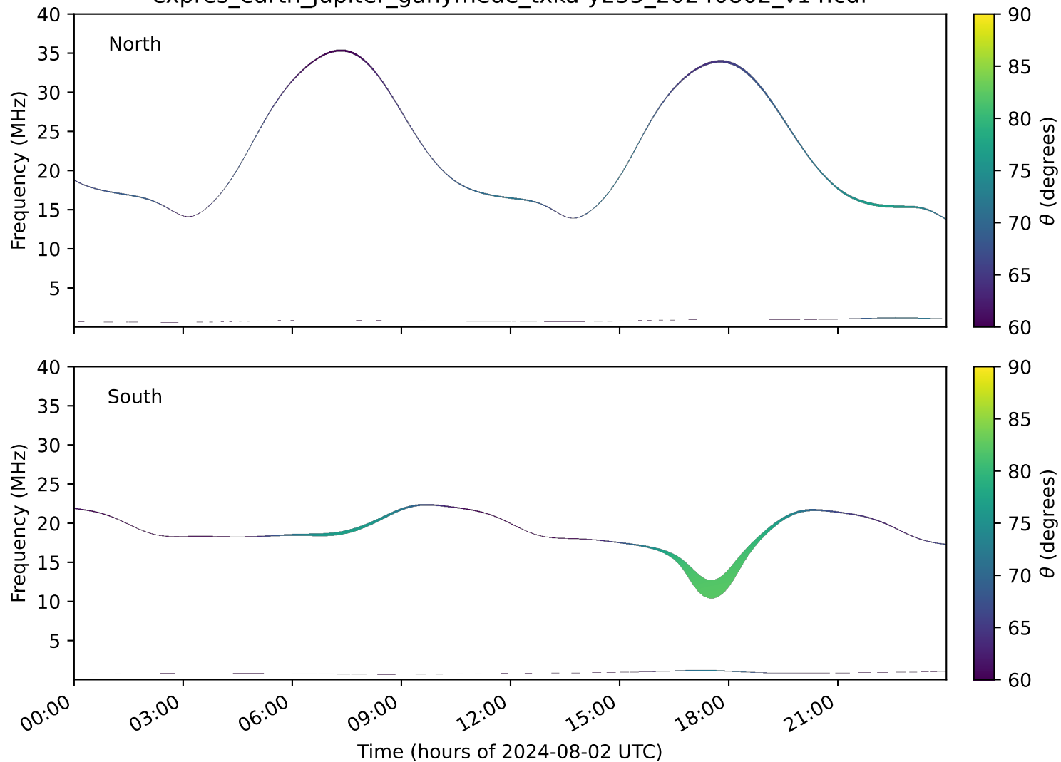
expres_earth_jupiter_ganymede_txka-y235_20240802_v14.cdf
