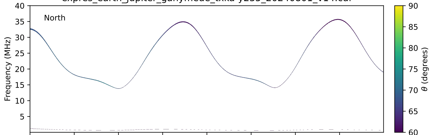
expres_earth_jupiter_ganymede_txka-y235_20240801_v14.cdf
