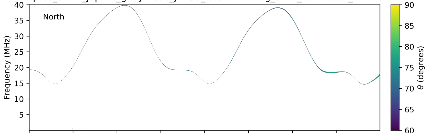
expres_earth_jupiter_ganymede_jrm33_lossc-wid1deg_3kev_20240831_v11.cdf
