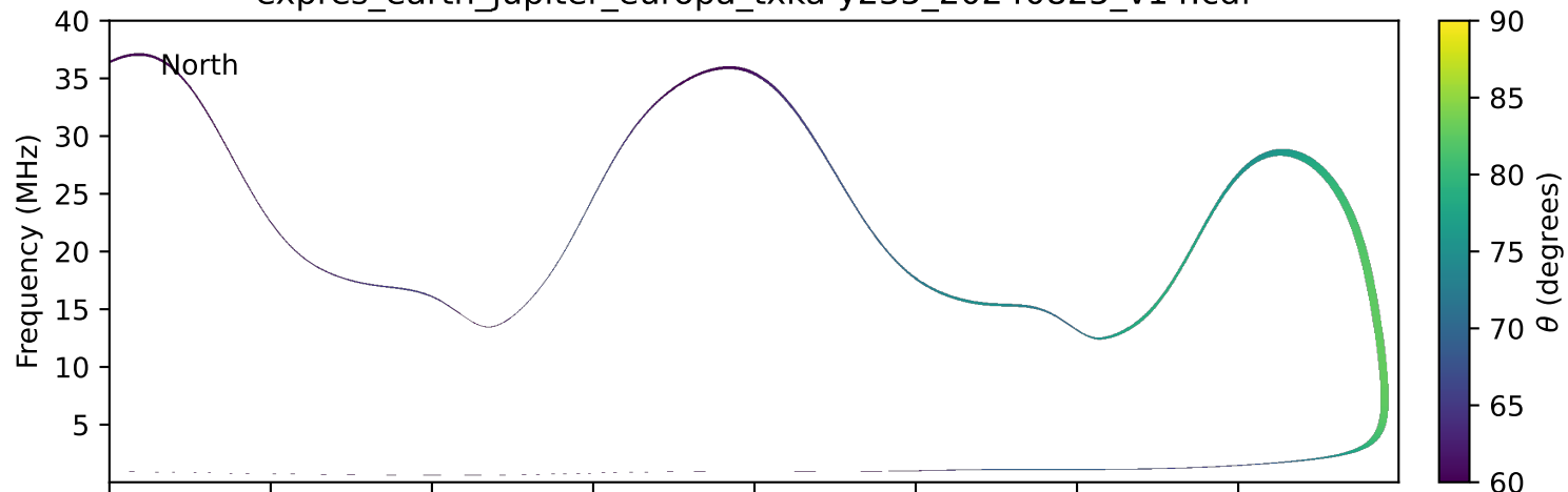
expres_earth_jupiter_europa_txka-y235_20240825_v14.cdf
