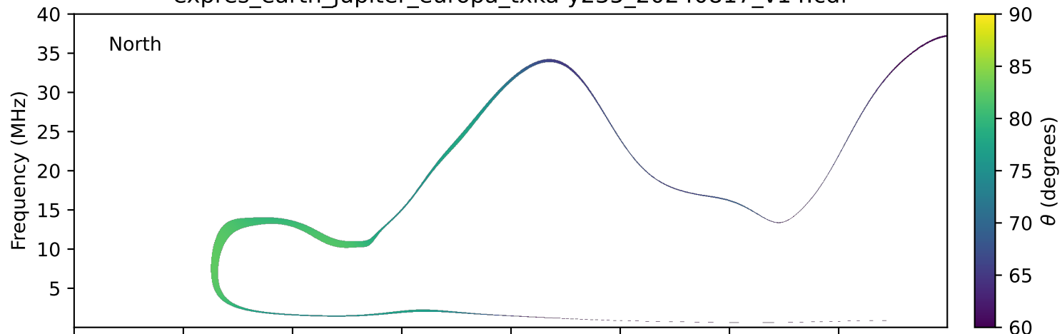
expres_earth_jupiter_europa_txka-y235_20240817_v14.cdf
