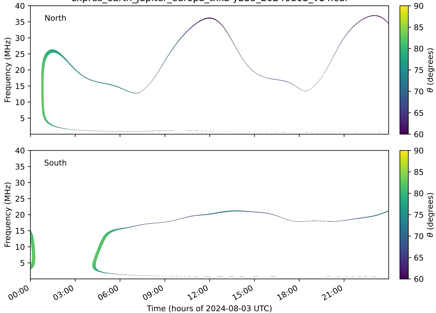
expres_earth_jupiter_europa_txka-y235_20240803_v14.cdf
