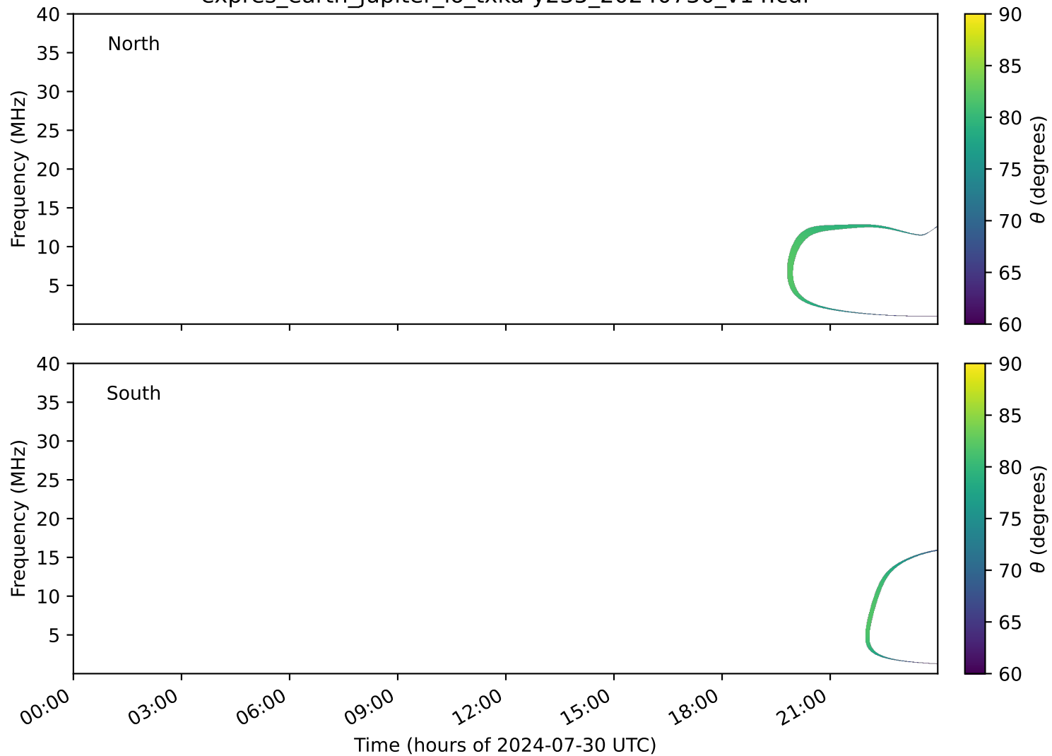
expres_earth_jupiter_io_txka-y235_20240730_v14.cdf
