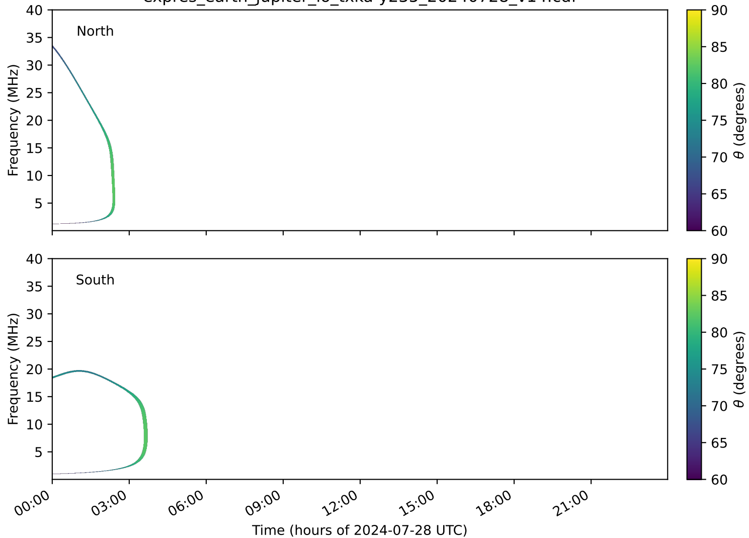
expres_earth_jupiter_io_txka-y235_20240728_v14.cdf
