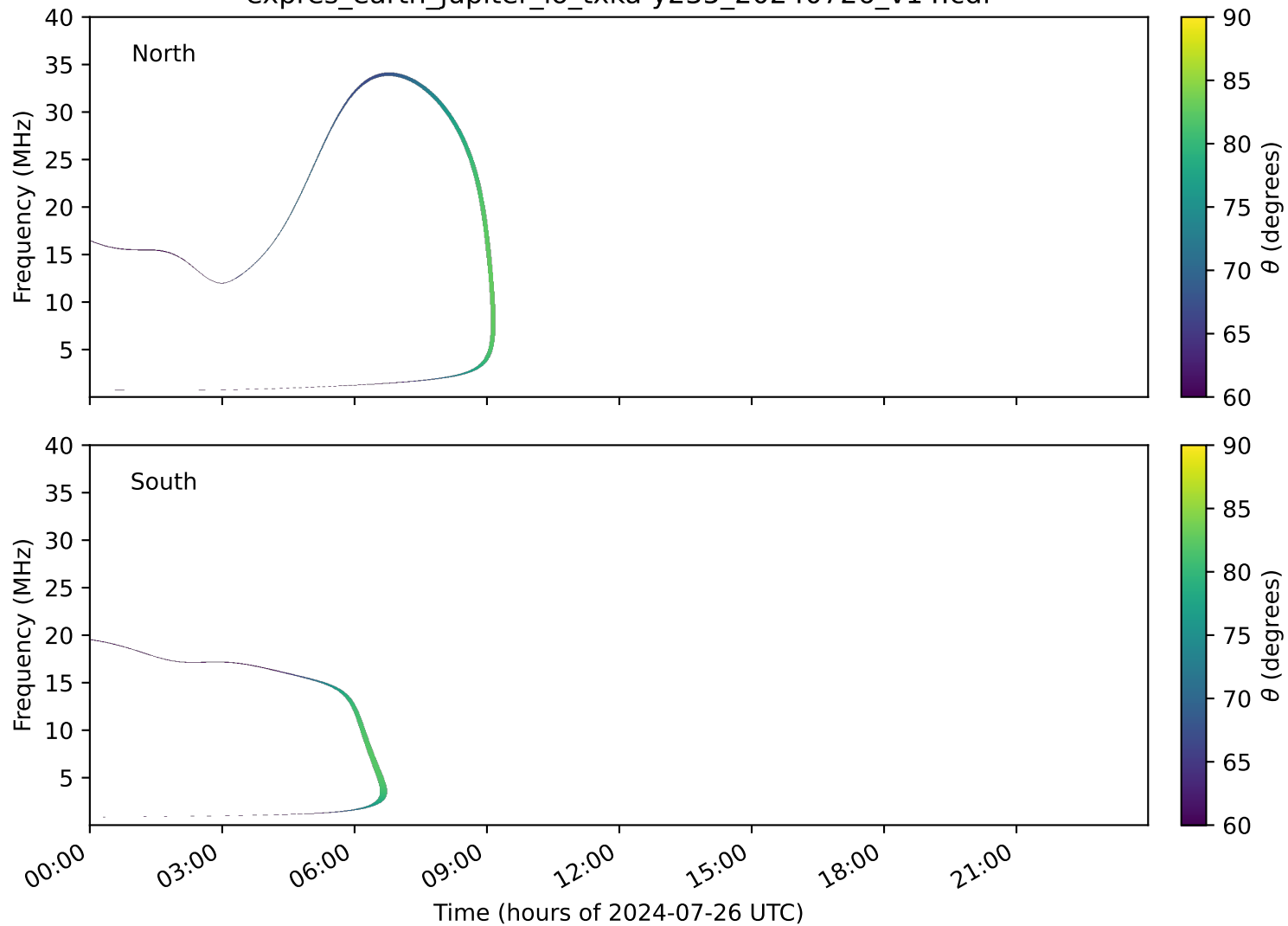
expres_earth_jupiter_io_txka-y235_20240726_v14.cdf
