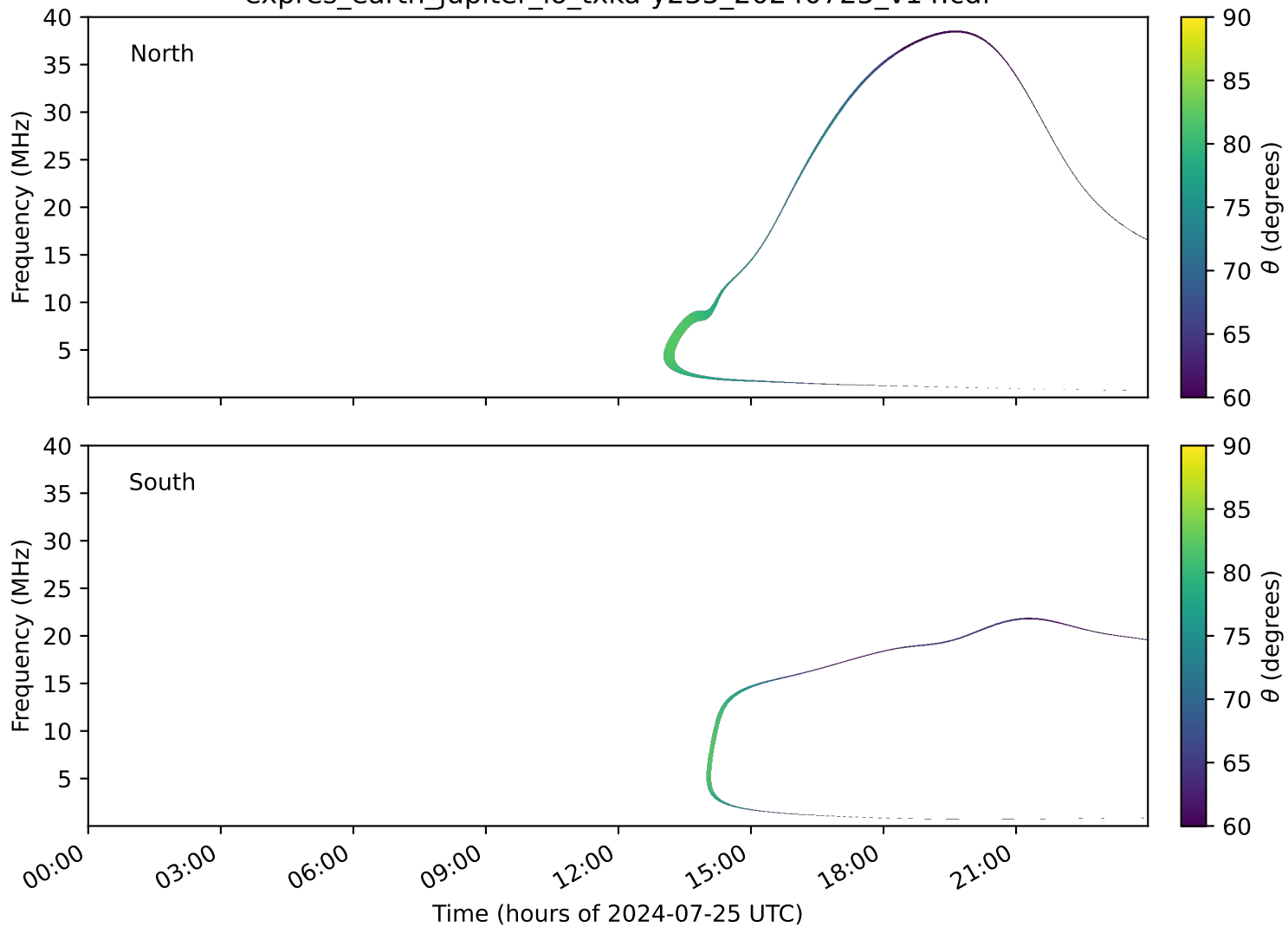
expres_earth_jupiter_io_txka-y235_20240725_v14.cdf
