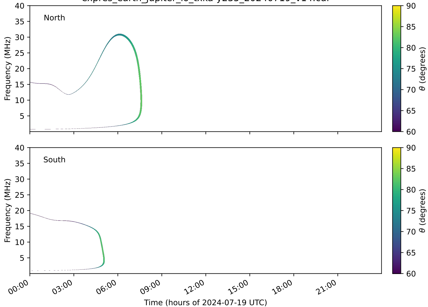
expres_earth_jupiter_io_txka-y235_20240719_v14.cdf
