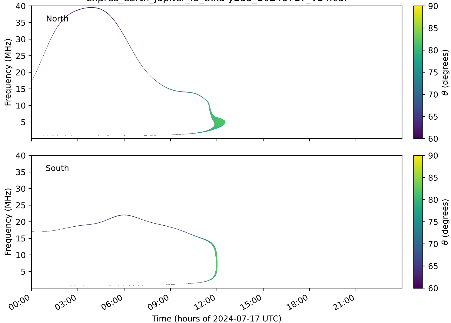
expres_earth_jupiter_io_txka-y235_20240717_v14.cdf
