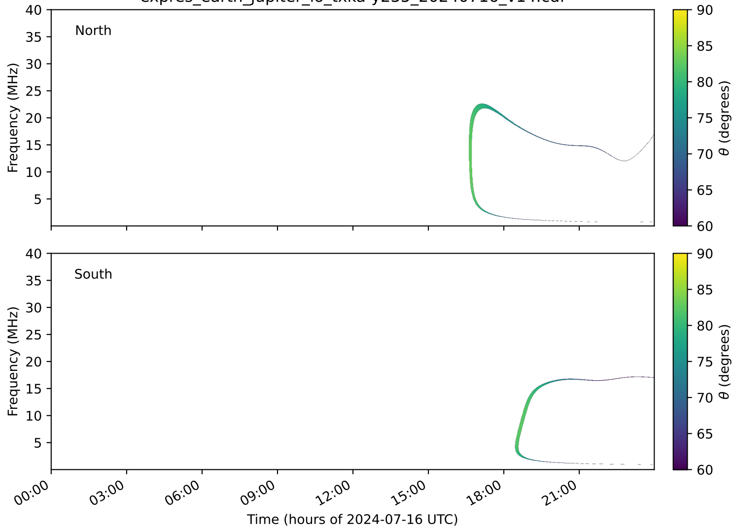
expres_earth_jupiter_io_txka-y235_20240716_v14.cdf
