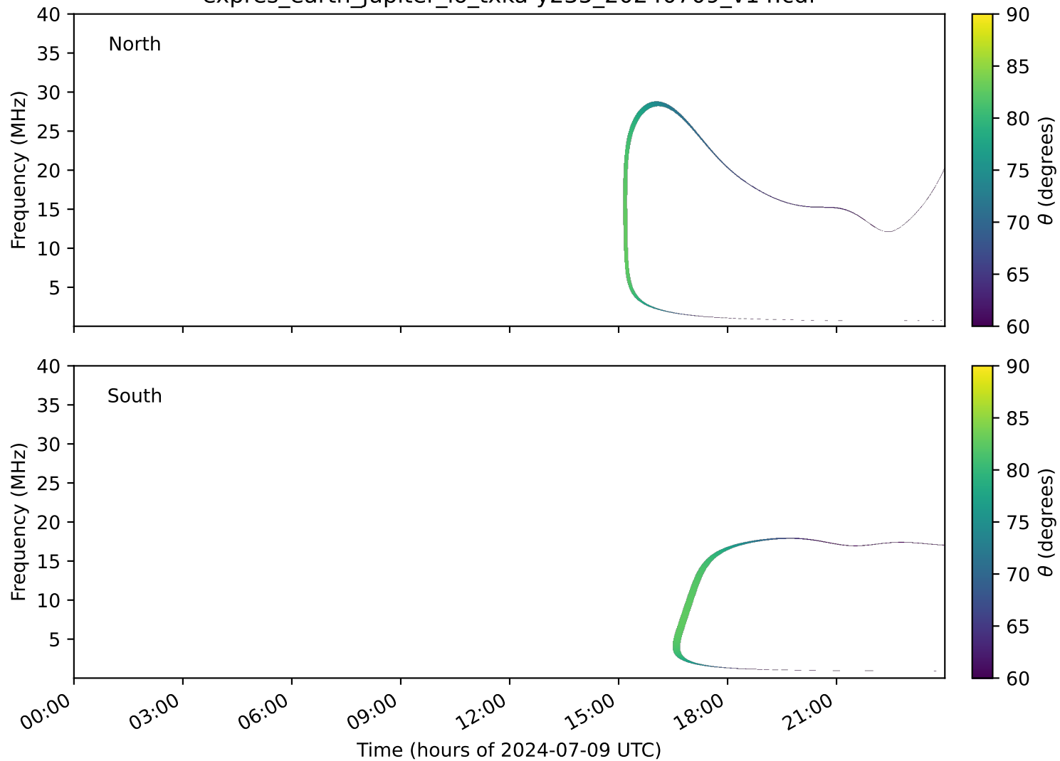
expres_earth_jupiter_io_txka-y235_20240709_v14.cdf
