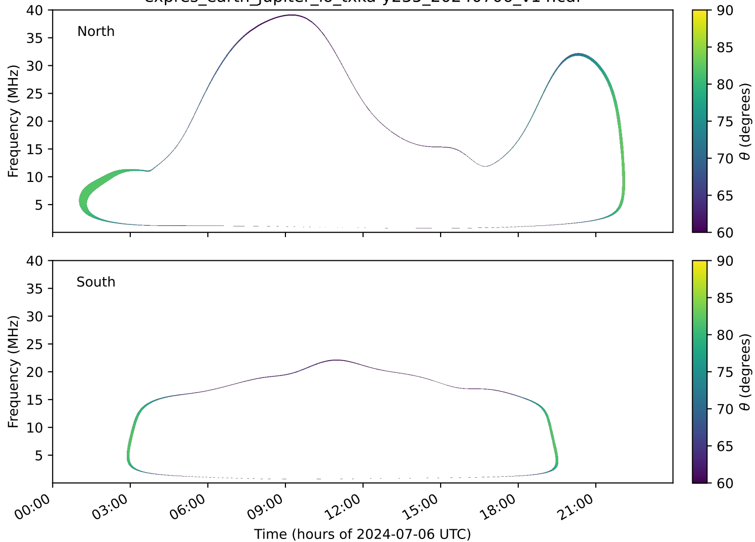
expres_earth_jupiter_io_txka-y235_20240706_v14.cdf
