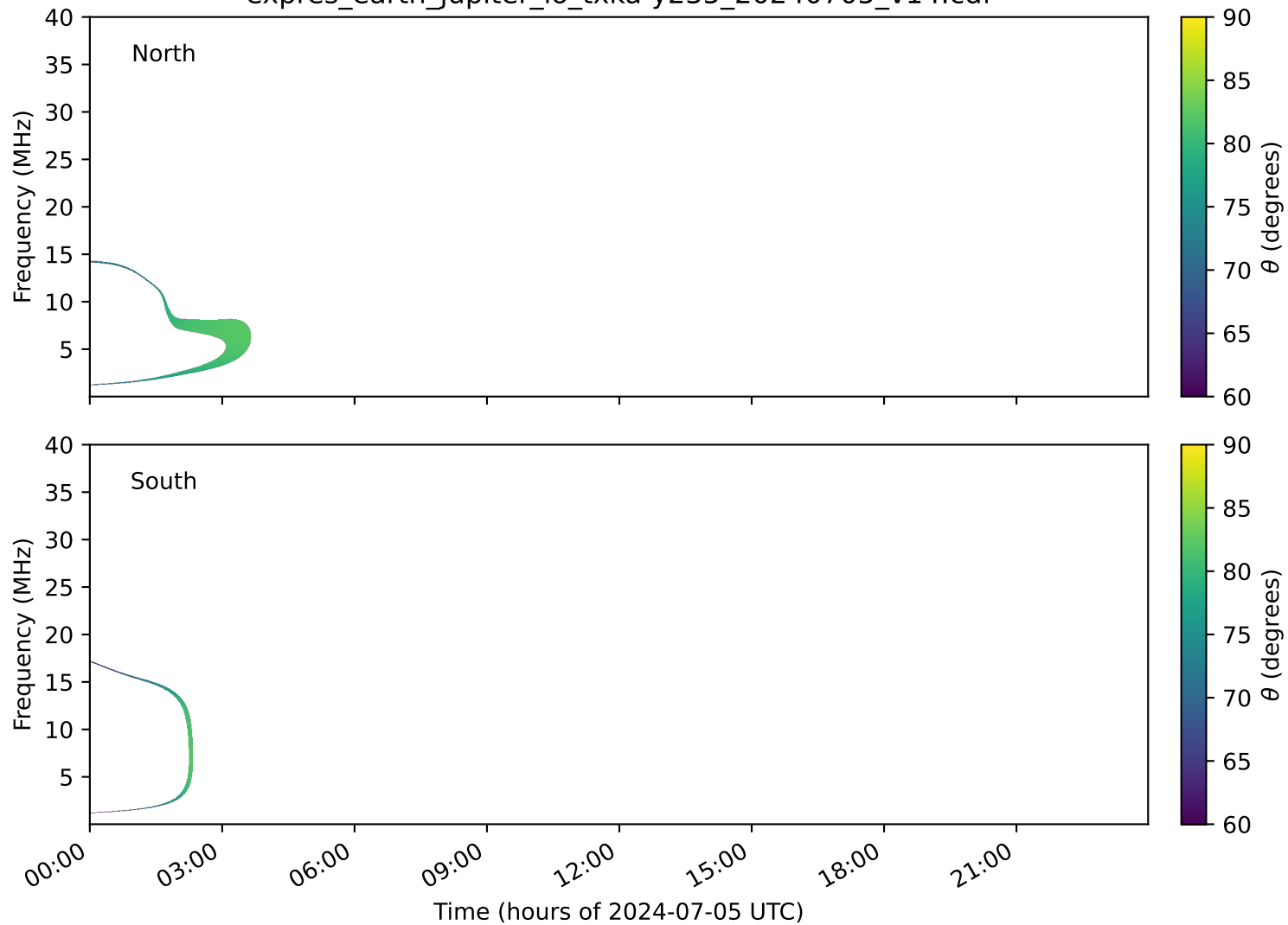
expres_earth_jupiter_io_txka-y235_20240705_v14.cdf
