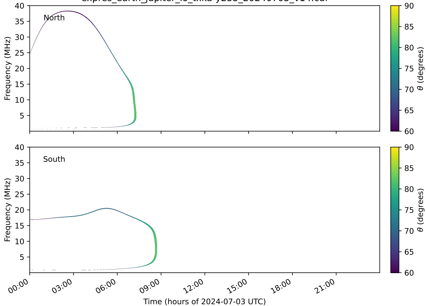
expres_earth_jupiter_io_txka-y235_20240703_v14.cdf
