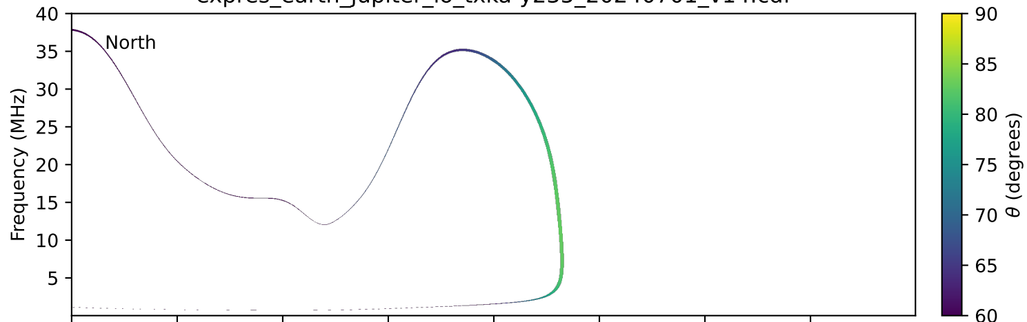
expres_earth_jupiter_io_txka-y235_20240701_v14.cdf
