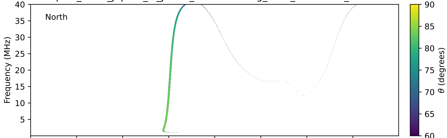
expres_earth_jupiter_io_jrm33_lossc-wid1deg_3kev_20240727_v11.cdf
