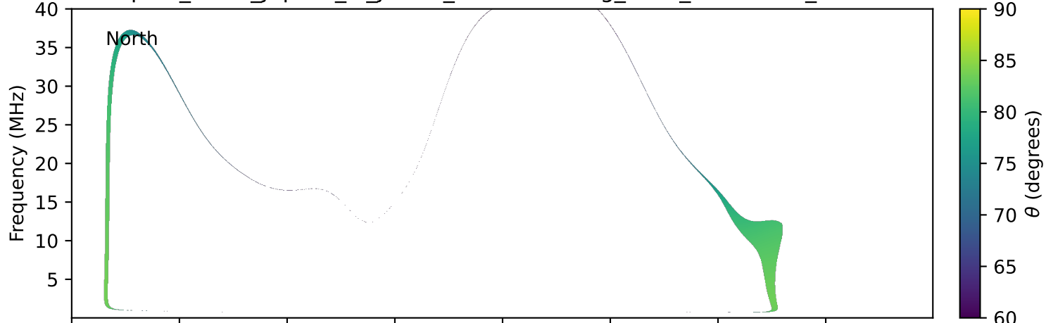
expres_earth_jupiter_io_jrm33_lossc-wid1deg_3kev_20240722_v11.cdf
