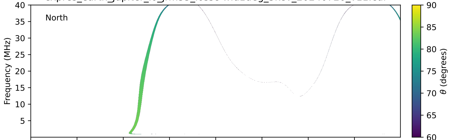
expres_earth_jupiter_io_jrm33_lossc-wid1deg_3kev_20240720_v11.cdf
