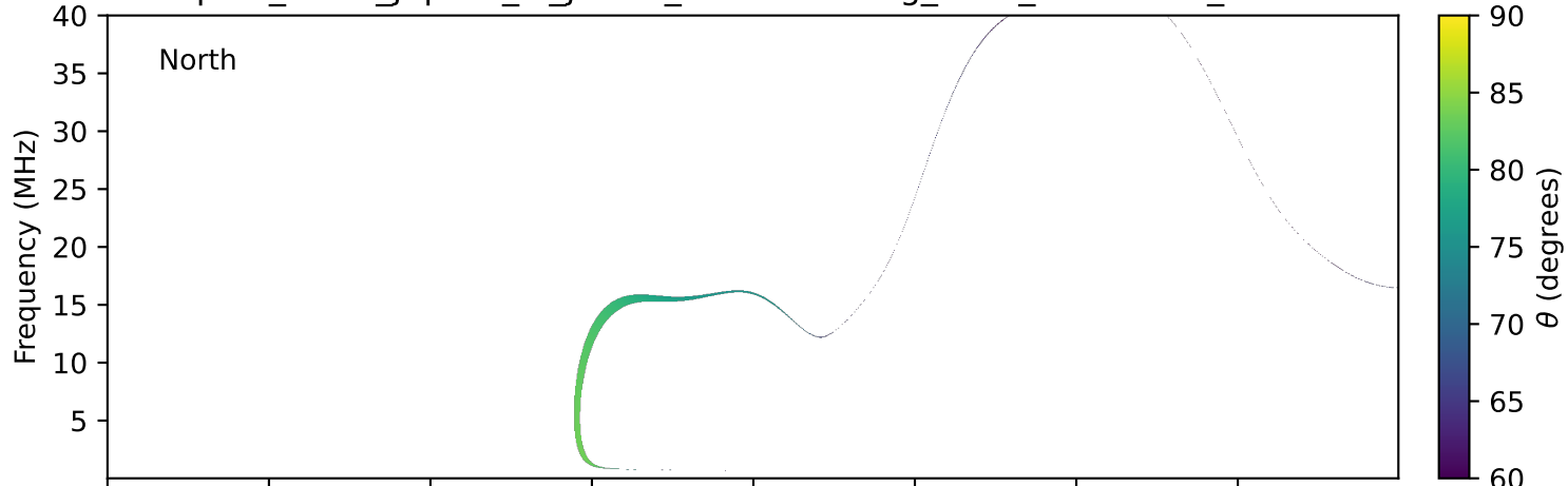
expres_earth_jupiter_io_jrm33_lossc-wid1deg_3kev_20240711_v11.cdf
