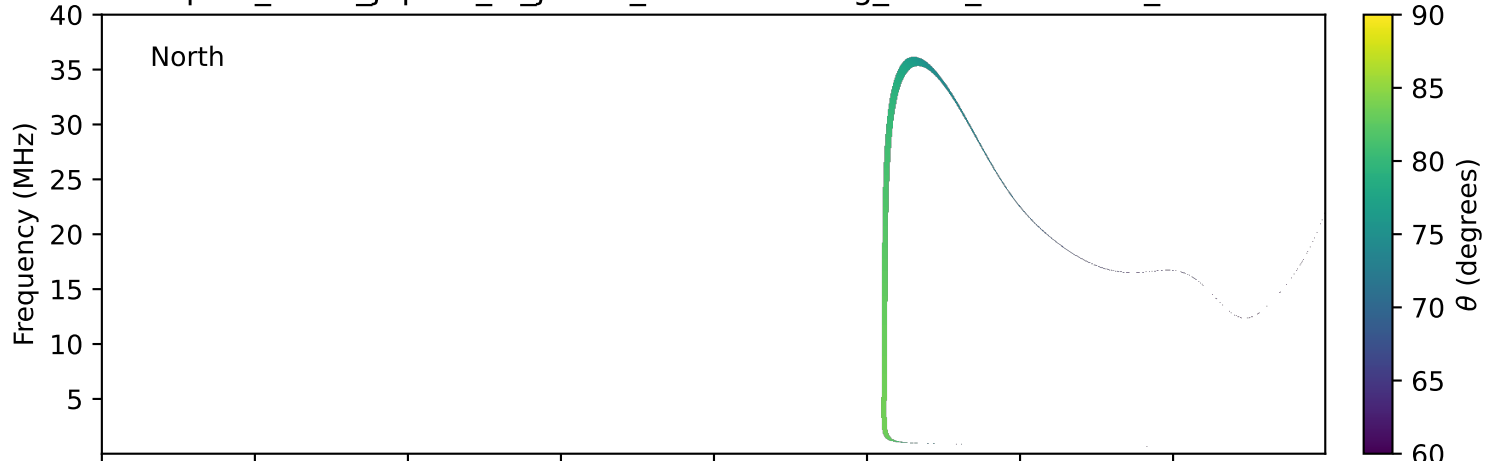
expres_earth_jupiter_io_jrm33_lossc-wid1deg_3kev_20240709_v11.cdf
