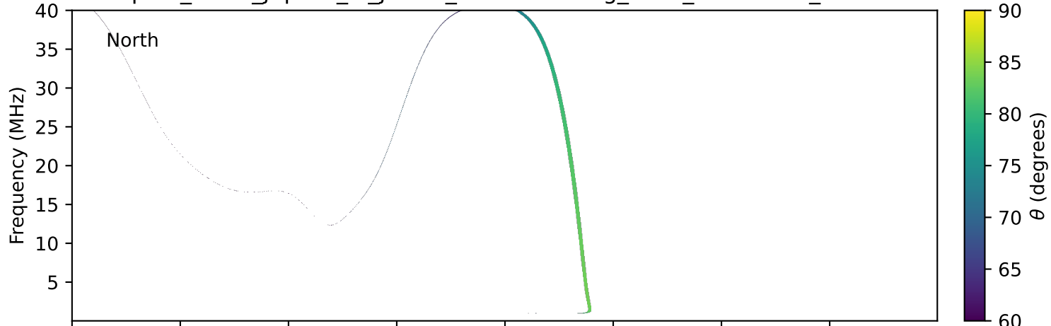
expres_earth_jupiter_io_jrm33_lossc-wid1deg_3kev_20240701_v11.cdf
